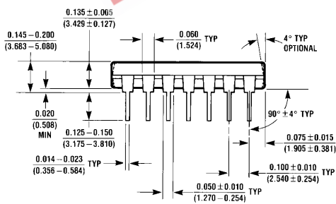
14-Lead Molded Dual-In-Line Package (N) Order Number DM74LS04N NS Package Number N14A
