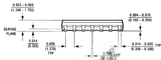
14-Lead Small Outline Molded Package (M) Order Number DM74LS04M NS Package Number M14A
